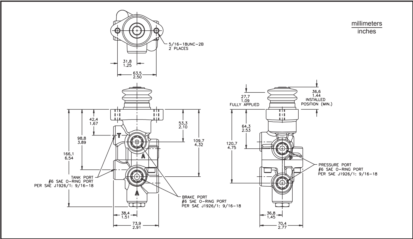
Typical Brake Valve
