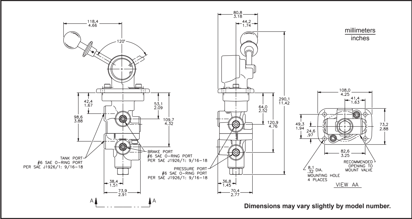
Typical Brake Valve
