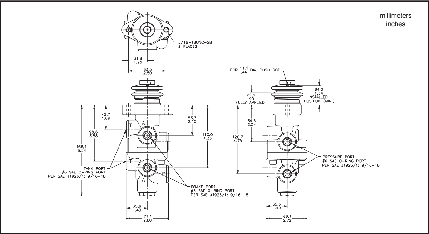
Typical Brake Valve
